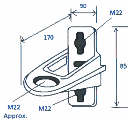
Fig. 4B: Typical Strain bracket
